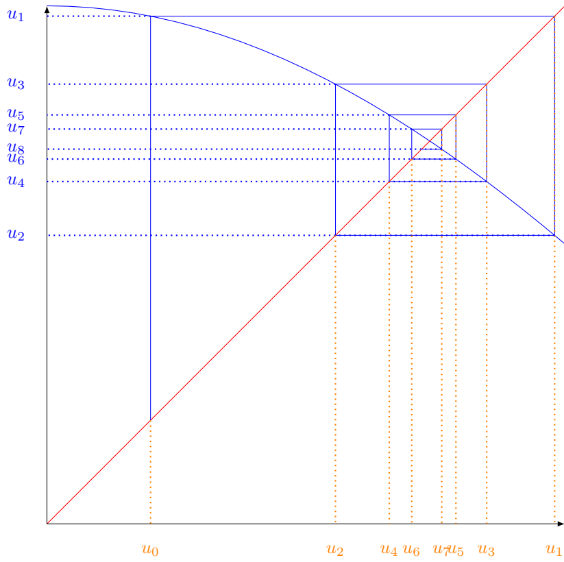
Figure 1: f(x) = \cos(x)
